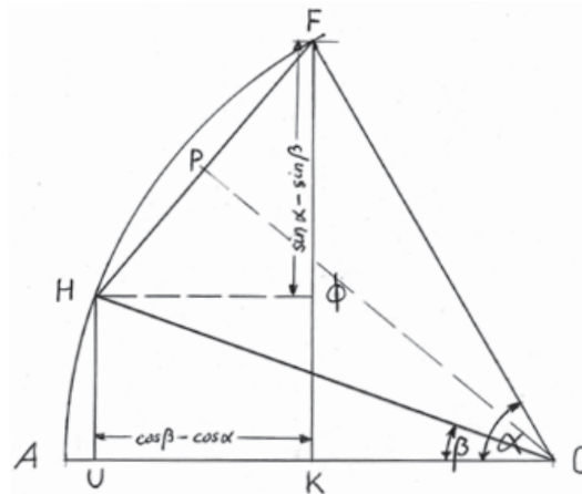
Abb. 73: Intersegment: \sin[(\alpha - \beta):2] .
